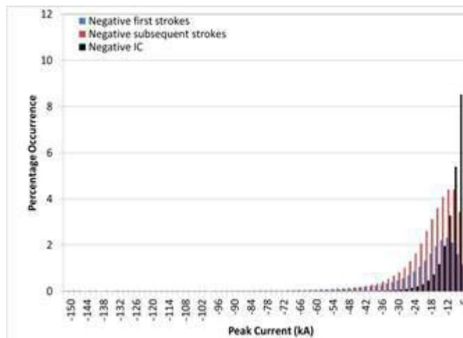
Figure 4. Histogram of NLDN-estimated peak current for negative and subsequent return strokes and cloud pulses shown in 2 kA bins. Note that the horizontal axis is truncated at -150 kA as the number of events having peak currents less than that value is smaller than 0.08%.
