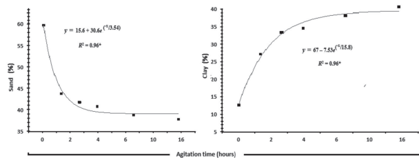
Figure 3. Curves and mathematical models that describe the trends of sand and clay fractions as a function of increasing in stirring time.
