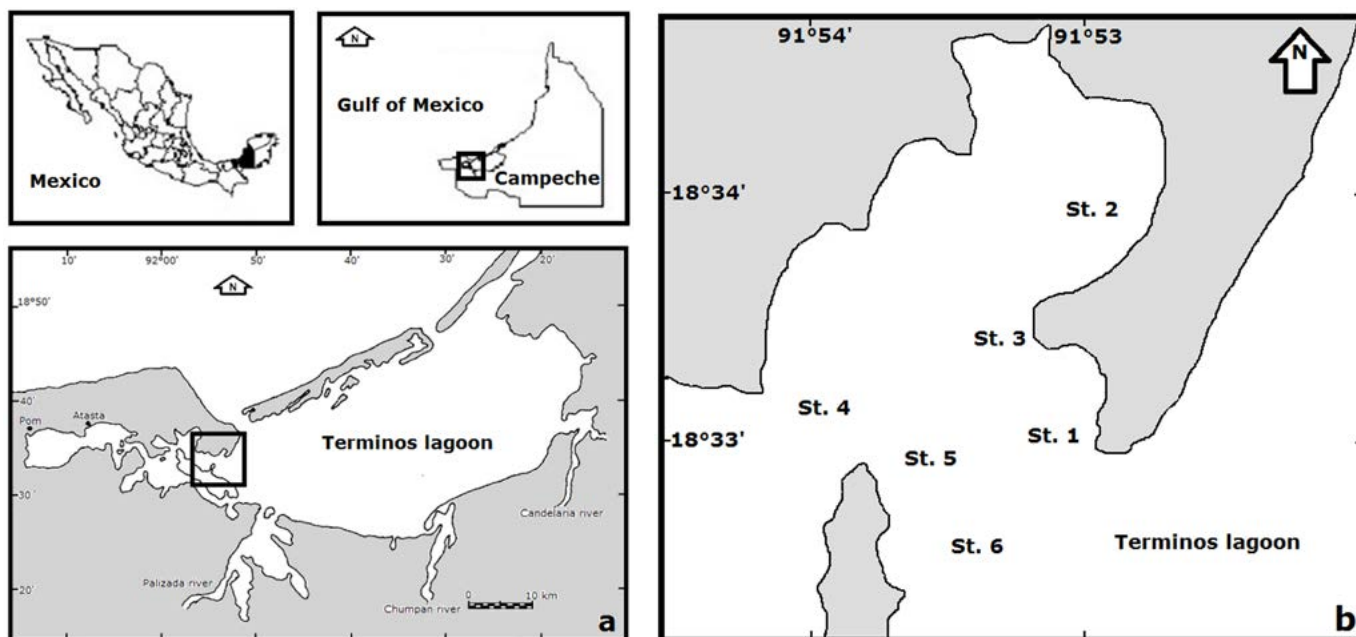
Figure 1. Study area: (a) the state of Campeche (shaded), Mexico, and (a, b) location of sampling stations in oyster banks (square).
