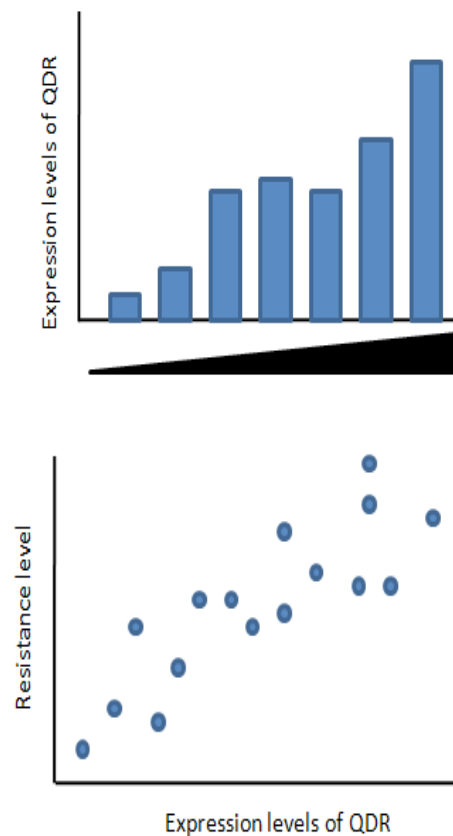
Figure 1. Model explaining the quantitative nature of resistance. As discussed in the text, the expression level of a group of particular genes involved in immunity contributes to the final output of the phenotype. The output intensity is determined by the number of genes induced and their expression level.
