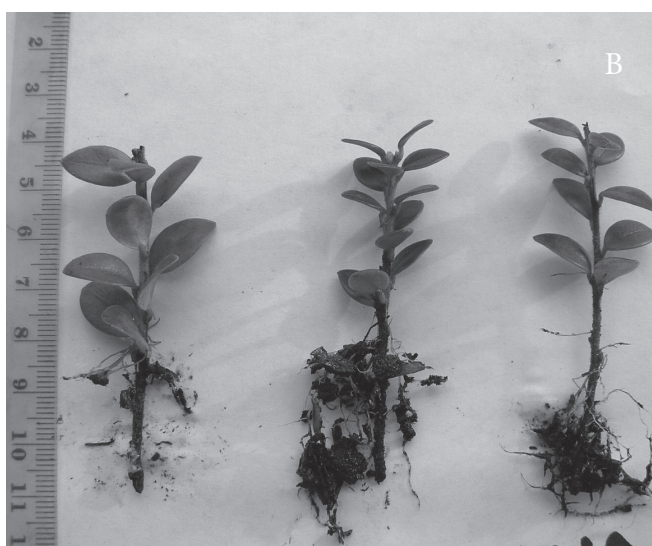
FIGURE 1. Rooting of young cuttings of V. floribundum (A) and D. alaternoides (B) after 60 days treated with 400 mg L -1 NAA.
