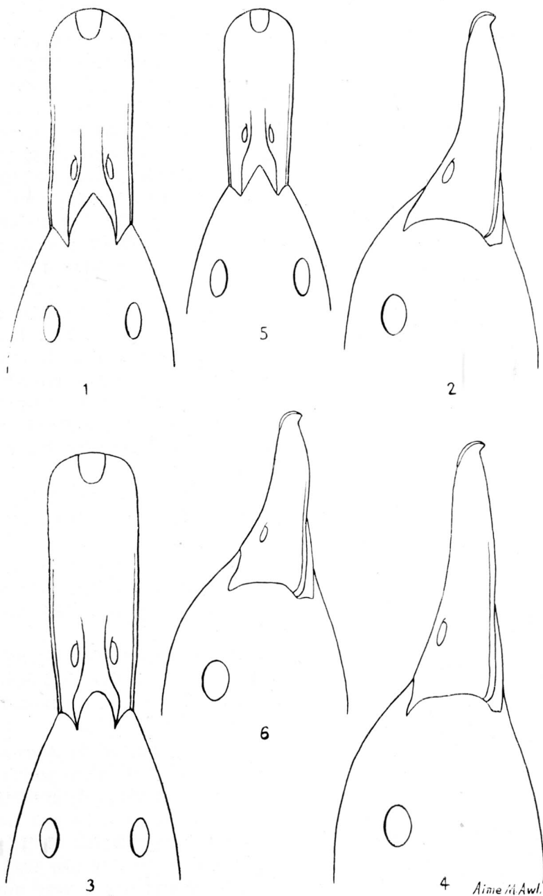
Figures 1-6. The bills of three related species of ducks of the genus Anas . 1-2 Anas spinicauda . 3-4 Anas niceforoi . 5-6 Anas georgica . (Slightly reduced).
