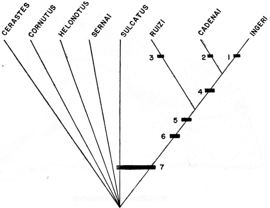
FIGURE 2. Cladogram of the species of the sulcatus group. Autapomorphies and synapomorphies are (1) narrowly separated cranial crests; (2) exostosis with bony papillae; (3) partial temporal arch; (4) bony cheek; (5) zygomatic process extending anteroventrally toward maxilla; (6) squamosal crests; (7) otic process of squamosal extending medially above the crista parotica.
