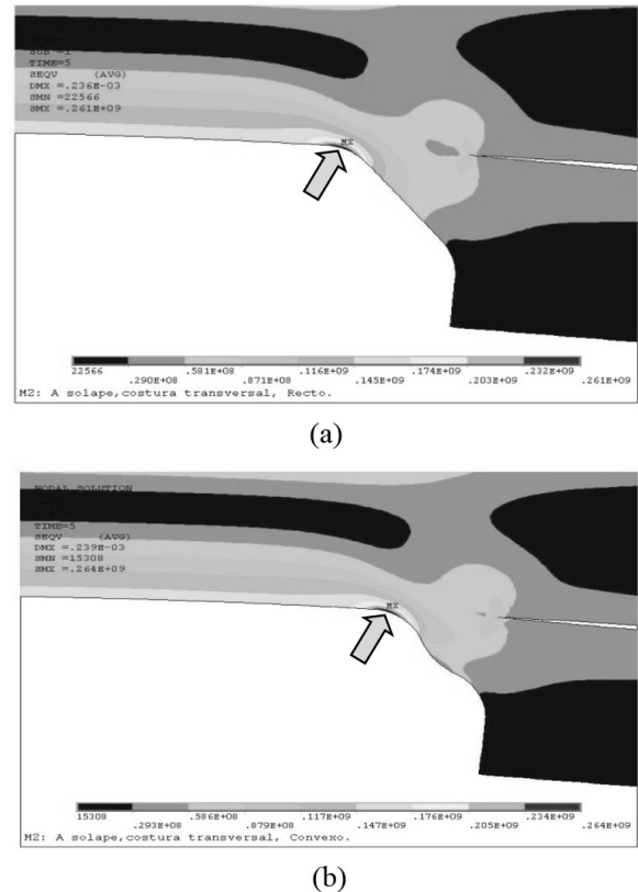
Figure 4. Post-processing results obtained for von Mises stresses. (a) straight bead profile; (b) convex bead profile
