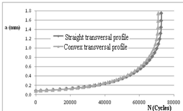
Figure 8. Stable crack propagation curves for both types of sections (eccentric crack; e/b=90\% )
