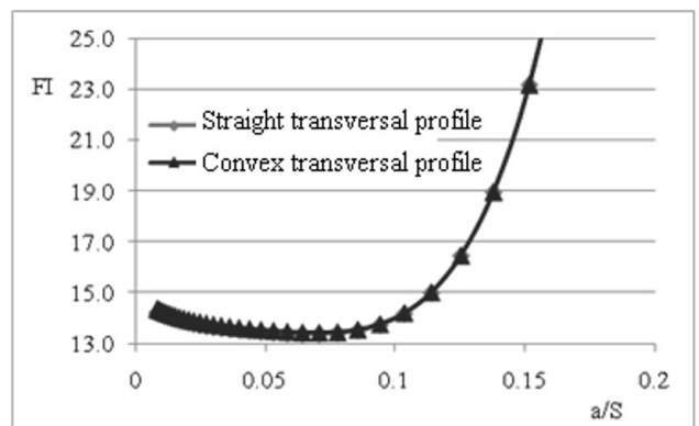
Figure 6. Dimensionless stress intensity factors for transversal crack with e/b=90\%
