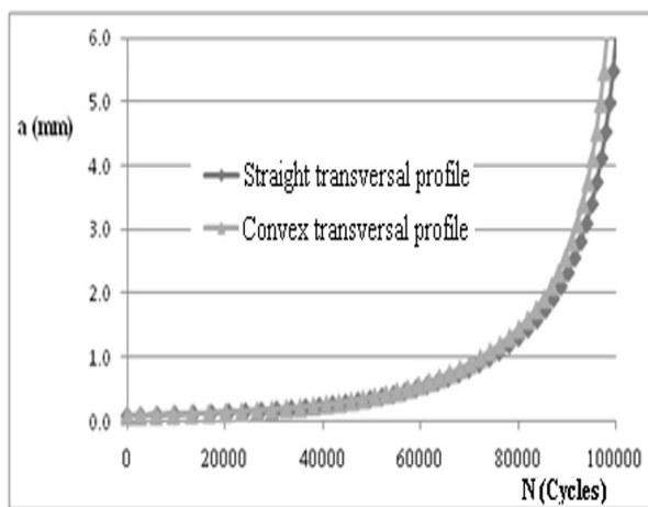
Figure 7. Stable crack propagation curves for both types of sections (central crack; e/b=0\% )
