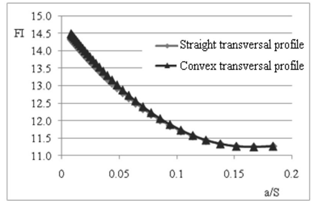
Figure 5. Dimensionless stress intensity factors for transversal crack with e/b=0\%
