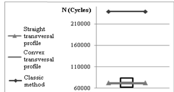
Figure 11. Comparative results among the proposed method, the classic method, and the experimental results
