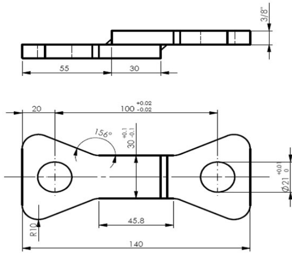
Figure 1. Geometry of the transversal fillet welding joint
