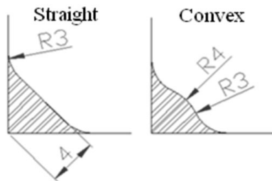
Figure 2. Profiles of weld beads employed in the modeling (measured in mm)
