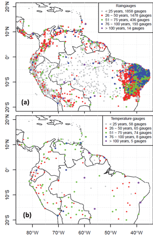
Figure 2. CLIMEXP ground stations in the Amazon region for (a) precipitation and (b) temperature data. Source: Authors' own compilation.
