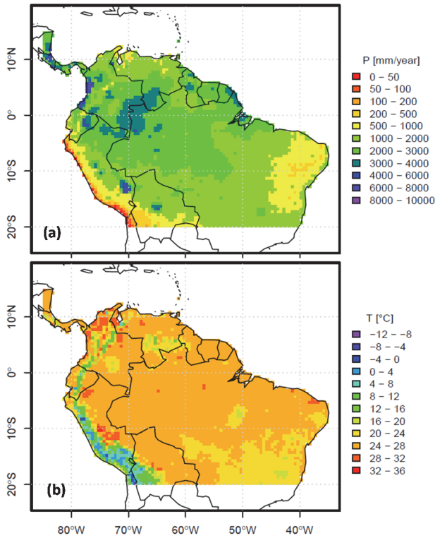
Figure 1. Yearly average (multi-year) for (a) precipitation and (b) temperature in the Amazon region, calculated using UD-ATP data (1950-2010 period). Source: Authors' own compilation.
