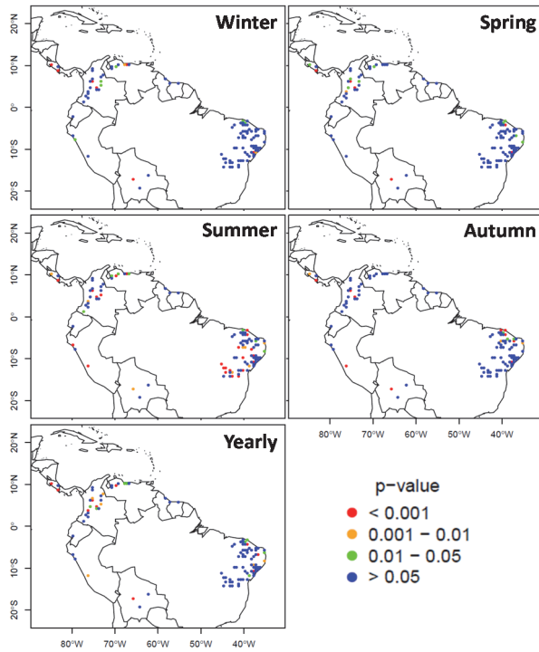
Figure 8. Maps of goodness-of-fit test results for precipitation, in seasonal and yearly terms, for pixels analyzed. Yearly division according with northern hemisphere seasons. Source: Authors' own compilation.
