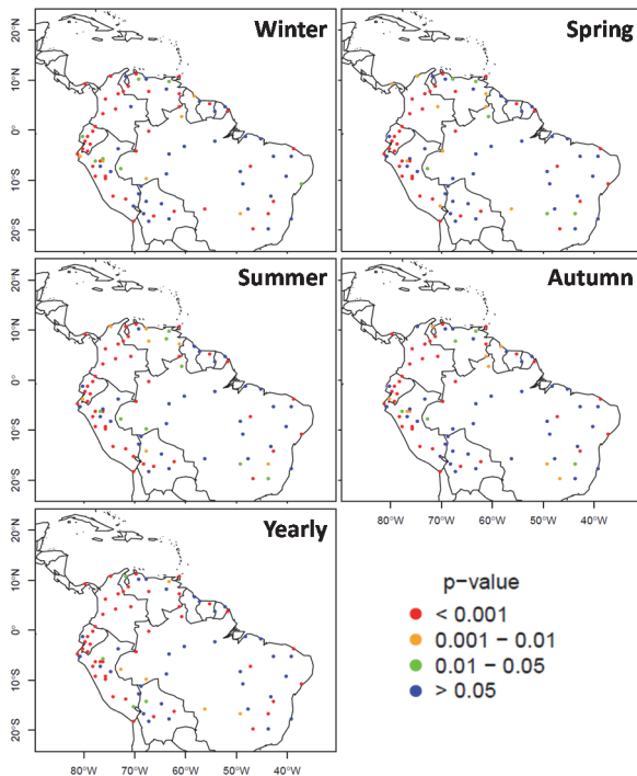
Figure 9. Similar to Fig. 8, but for temperature. Yearly division according with northern hemisphere seasons. Source: Authors' own compilation.
