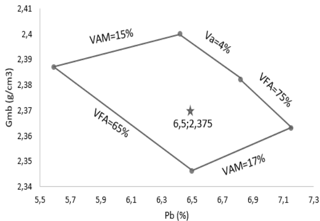
Figure 4. The polygon of voids for the M2 mixture
