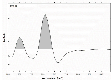
Figure 7. Area of the vibration signals at 720 cm -1 for the three EVA polymers. Source: The Authors.
