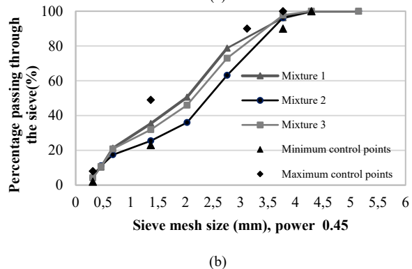
Figure 2. Particle size curves of the trial mixtures of mineral aggregates used in the Superpave design method and respective classifications in the limits of the gradation B of DNIT (a) and in the control point requirements (b).
