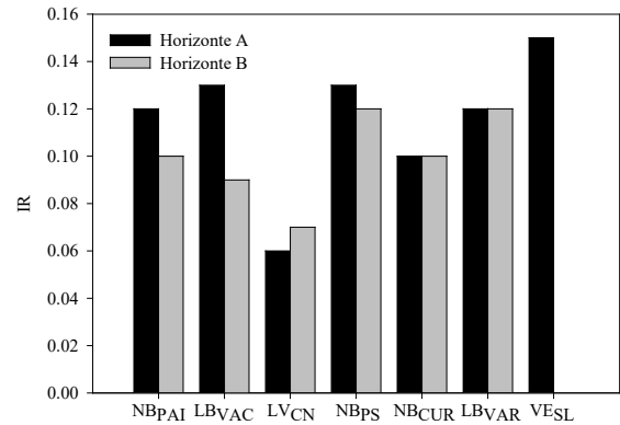
Soil horizons
