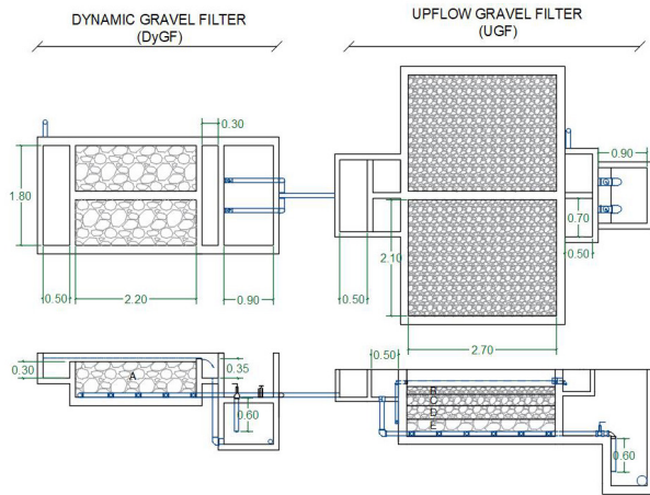
Figure 1. Scheme of treatment plant and gravel size
