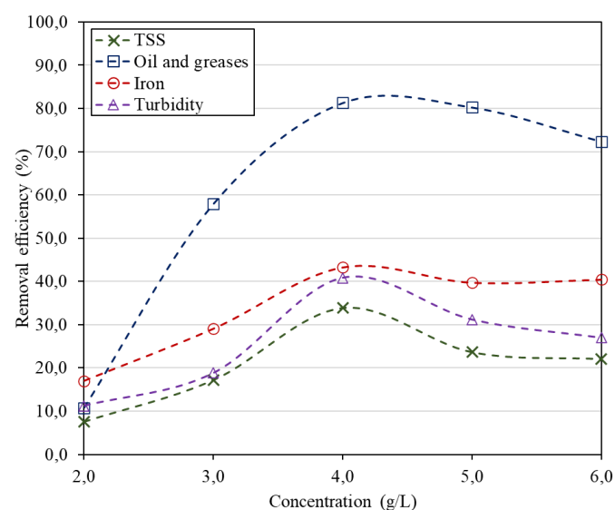
Figure 1. Removal efficiency of Moringa coagulant for total suspended solids, oil and greases, iron, and turbidity from produced water
