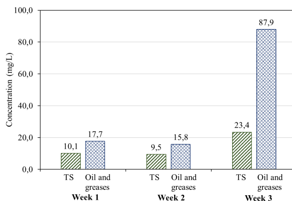
Figure 2. Quantity of total suspended solids and oil and greases in the produced water samples collected over three consecutive weeks from the oil reservoir
