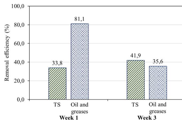
Figure 3. Efficiency of Moringa oleifera coagulant in removing total suspended solids and oil and greases from produced water samples collected during weeks 1 and 3
