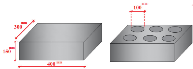
Figure 1. Schematic of the produced concrete masses Source: Authors
