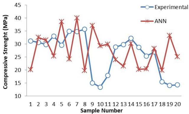
Figure 11. Compressive strength comparison chart for real buildings (experimental-ANN)
