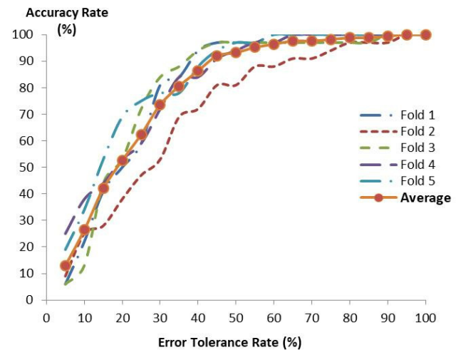
Figure 10. Accuracy of 5-fold cross validation results for the test set
