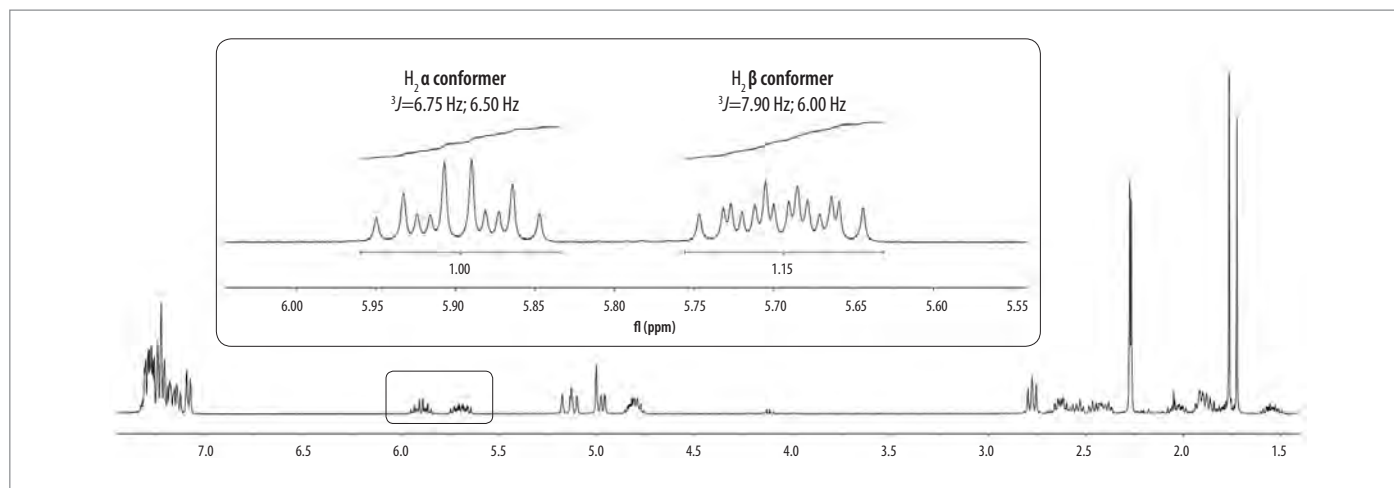
Figure 3. 1 H-NMR (CDCl 3 , 400MHz) spectra of 2f ; the two different allyl-H 2 signals (in expansion) determine the α/β conformers.
