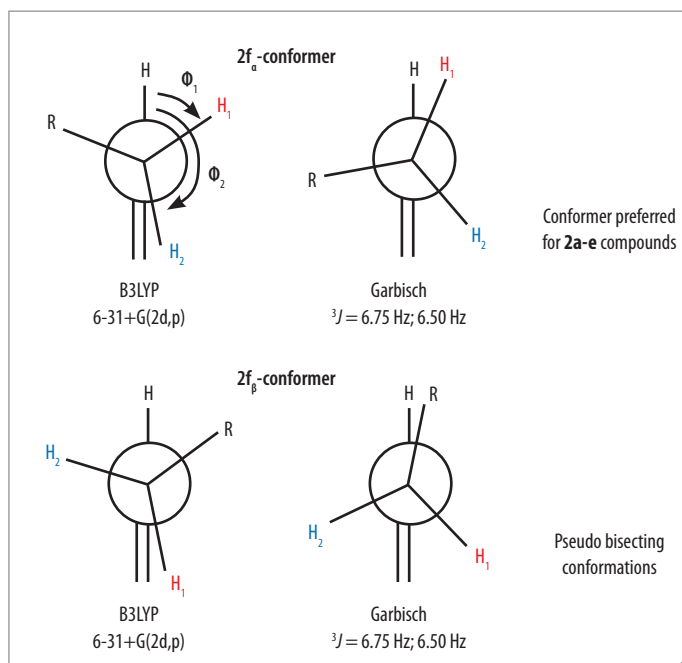
Figure 5. Newman projections for allyl group conformers 2f \alpha and 2f \beta : left, calculated structures (B3LYP/6-31+G(2d,p)); right, according to [Equation 1].
