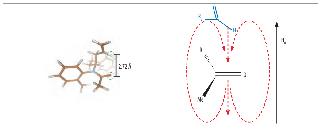
Figure 7. Left: Allyl- H_2 proton interaction at 2.72 Å distance with the carbonyl oxygen in conformer 2f β . Right: The diamagnetic protection zone of double bond C=O.
