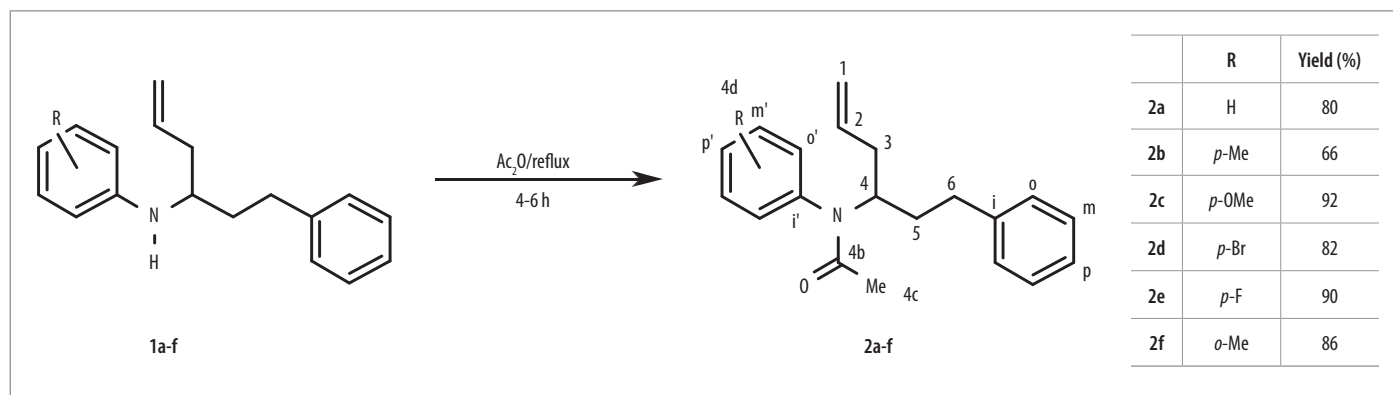
Figure 1. Synthesis of acetamides 2a-f (see labels for 1 H/ 13 C-NMR assignments in experimental section).
