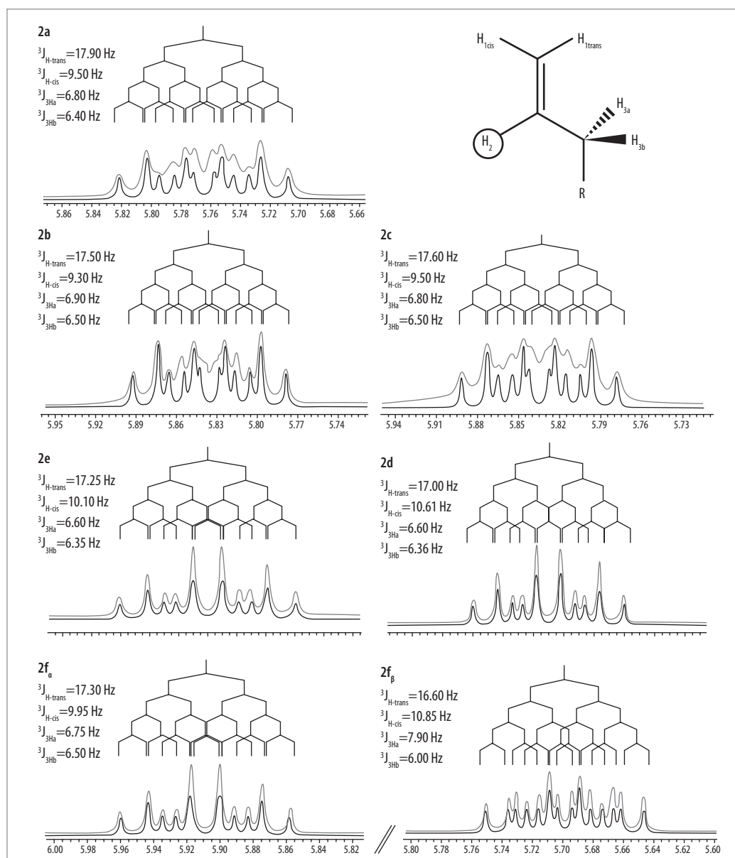
Figure 2. Obtained (gray) and simulated (black) spectra for allyl- H_2 proton considering an AA'MXX' spin system.
