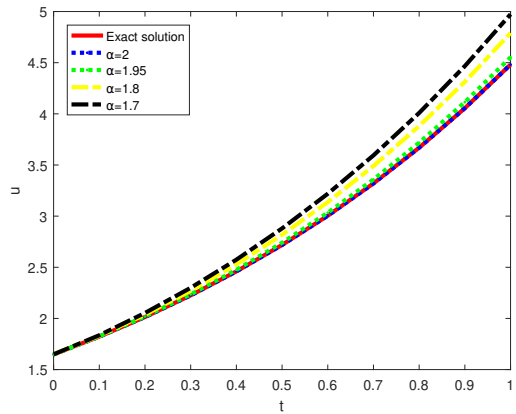
FIGURE 4. 2D plots for the 4-term approximate solution by SHAM and exact solution for equations (38) and (39) when h = -1 and x = 0.5
