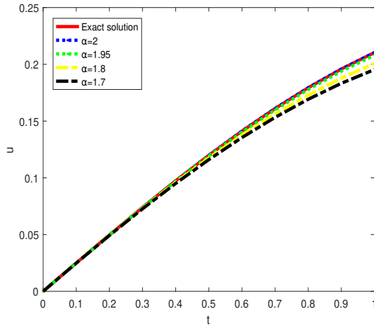
FIGURE 6. 2D plots for the 4-term approximate solution by SHAM and exact solution for equations (47) and (48) when h = -1 and x = 0.5
