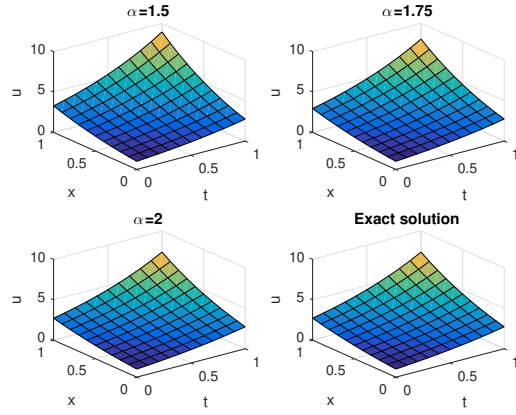
FIGURE 3. 3D plots for the 4-term approximate solution by SHAM and exact solution for equations (38) and (39) when h = -1
