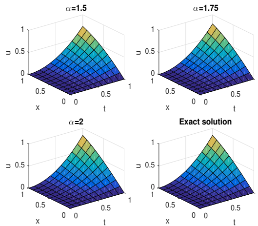
FIGURE 5. 3D plots for the 4-term approximate solution by SHAM and exact solution for equations (47) and (48) when h = -1
