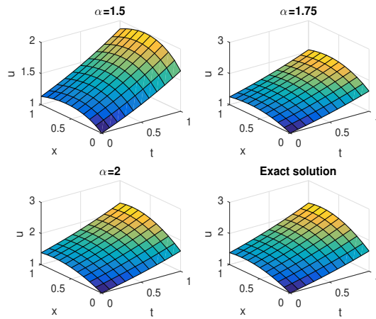
FIGURE 1. 3D plots for the 4-term approximate solution by SHAM and exact solution for equations (28) and (29) when h = -1 and y = 0.5
