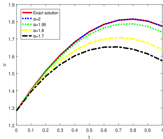
FIGURE 2. 2D plots for the 4-term approximate solution by SHAM and exact solution for equations (28) and (29) when h = -1 and x = y = 0.5
