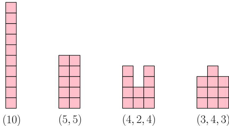
FIGURE 1. Palindromic compositions of n = 10 .
