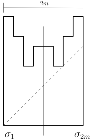
FIGURE 2. Decomposition of a palindromic superdiagonal composition.
