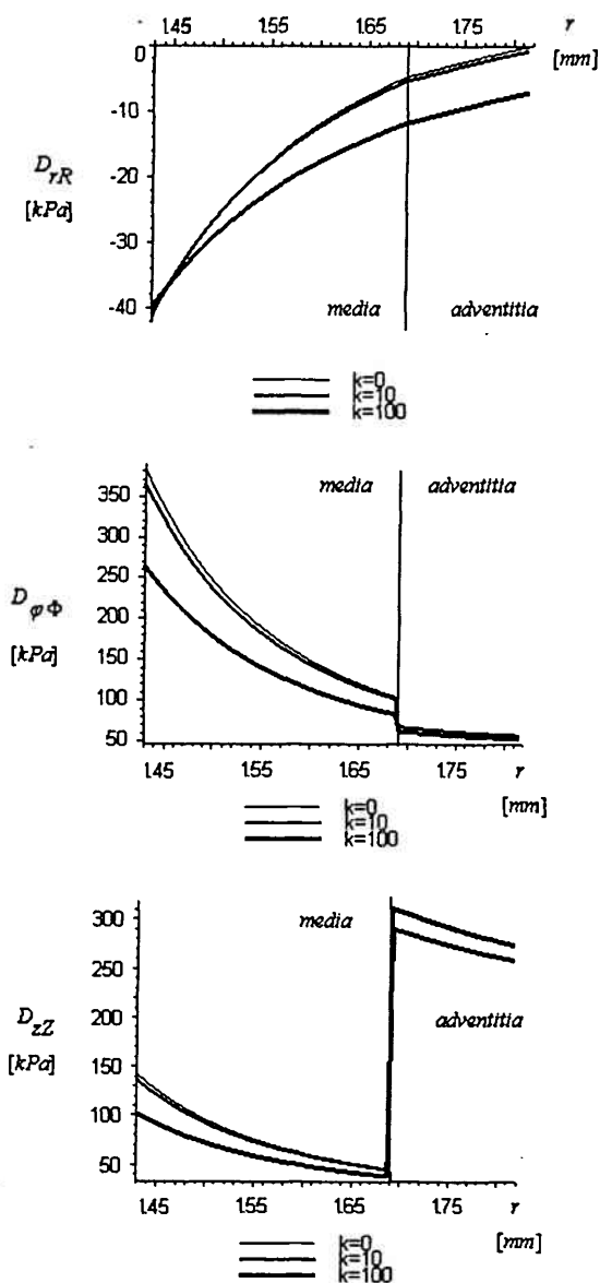
FIGURE 3. Distribution of normal stresses on the radius of the cylinder for various values of k when \lambda = 1.9 .
