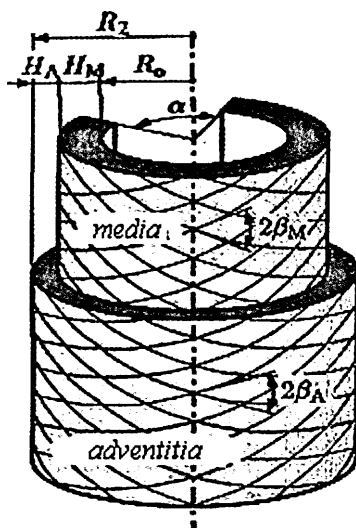
FIGURE 1. An artery as a two-layer cylinder.
