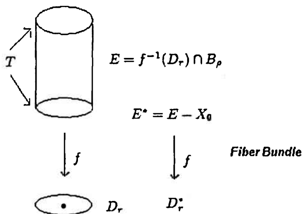
FIGURE 5. Milnor's picture seen abstractly.
